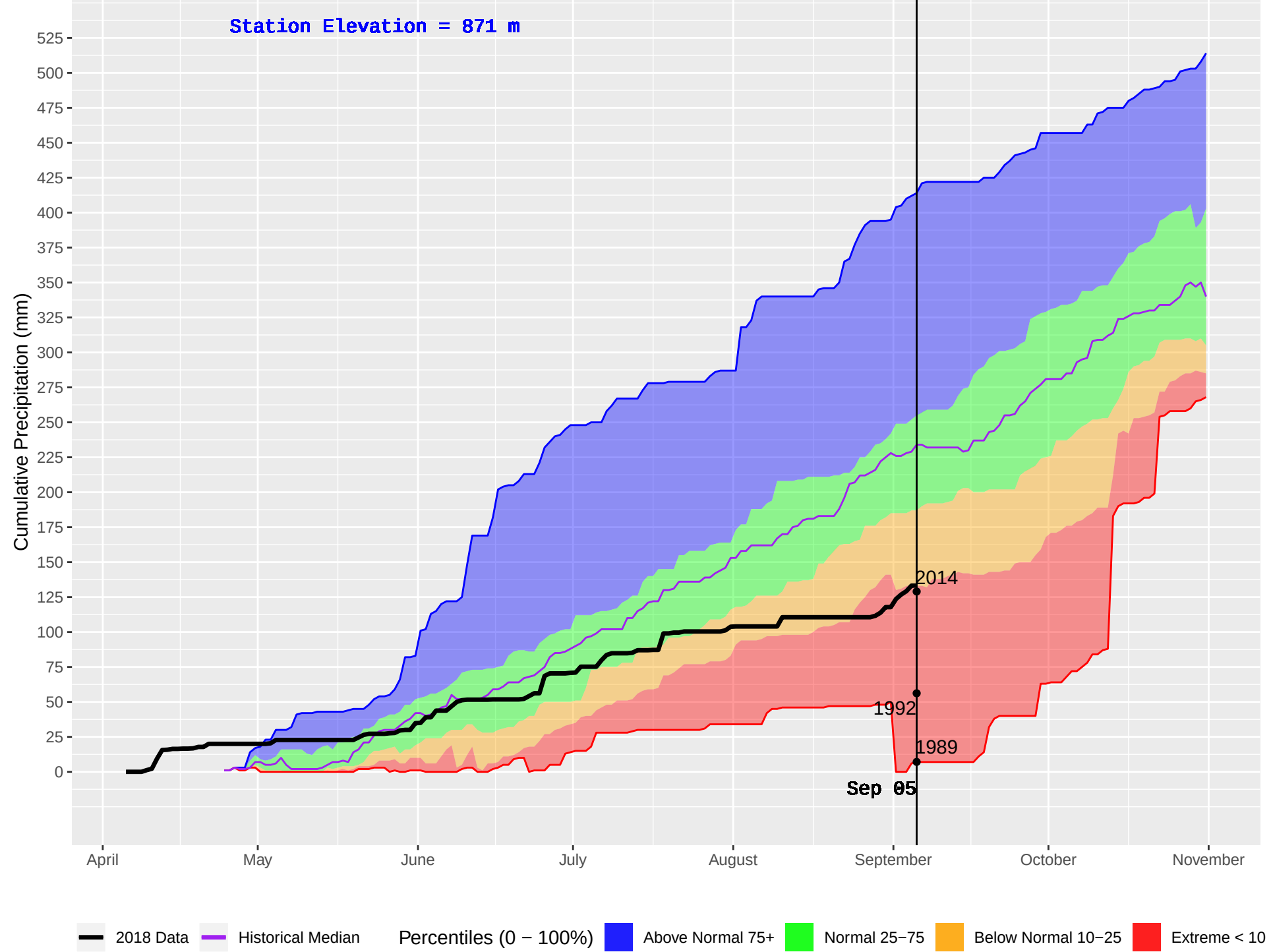
SUSTUT (156) : Historical (1989–2016) and Current (2018) Daily Cumulative Precipitation
